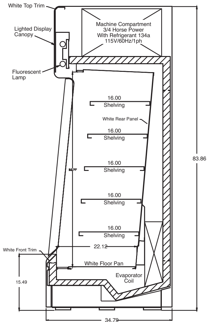
Cross Section
