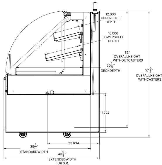
CROSS SECTION
