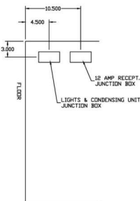
JUNCTION BOX
