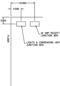
JUNCTION BOX
