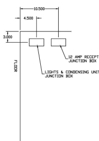
JUNCTION BOX
