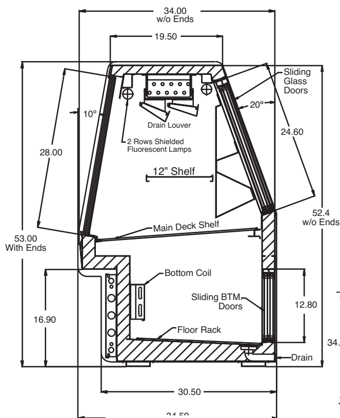
Cross Section
