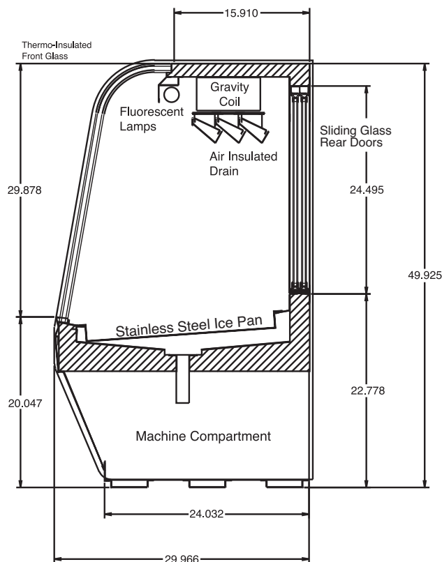
CROSS SECTION
