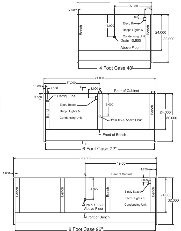
PLAN VIEWS
