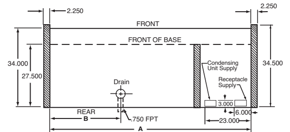
PLAN VIEWS
