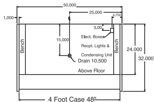
PLAN VIEWS
