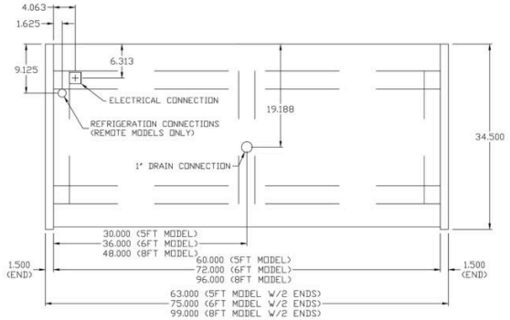
5/6/8 FOOT MODEL
