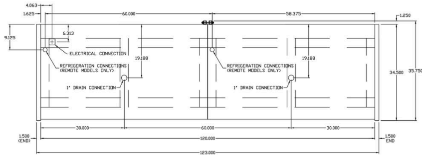
10 FOOT MODEL
