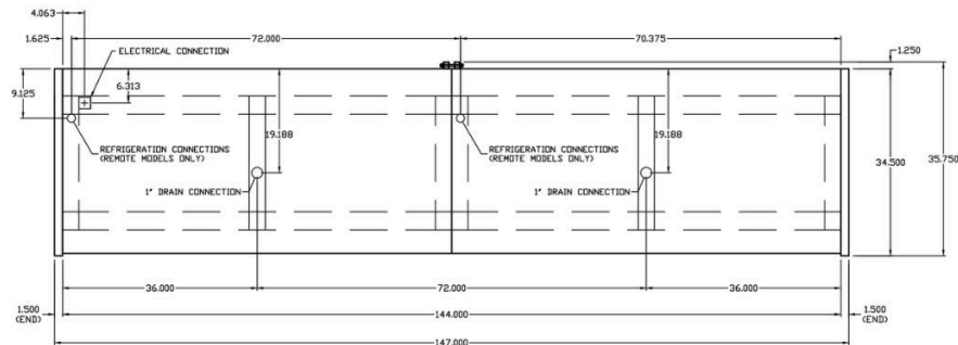
12 FOOT MODEL
