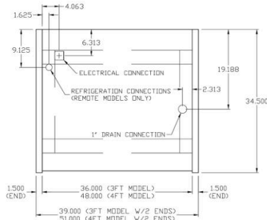
3/4 FOOT MODEL
