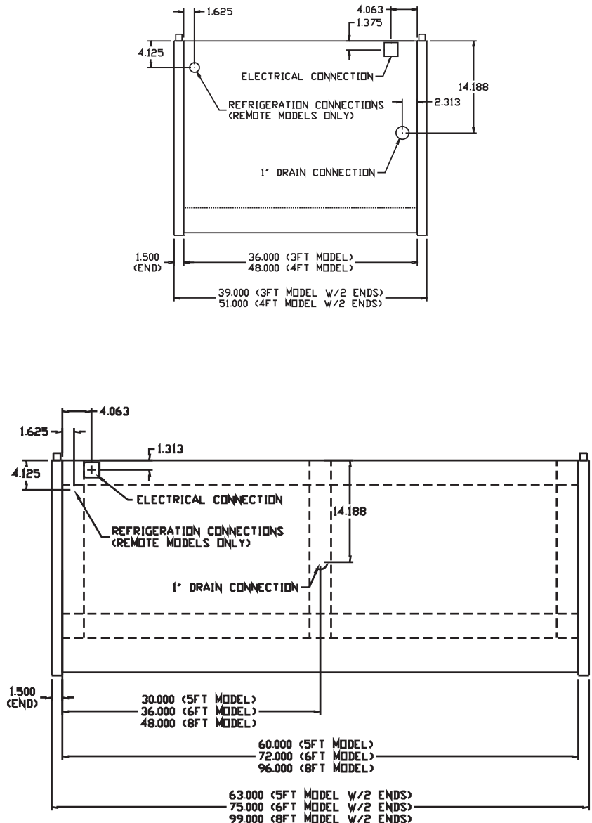
PLAN VIEWS
