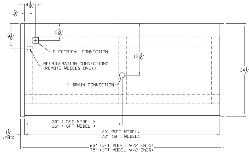
PLAN VIEW (5' & 6')
