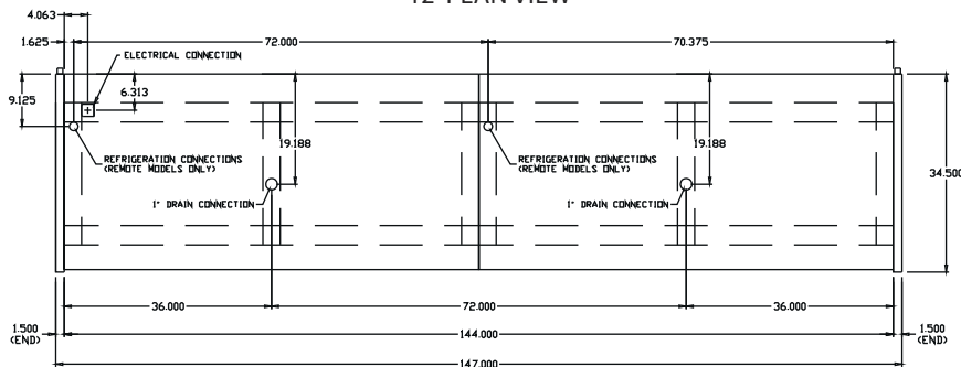
12' PLAN VIEW
