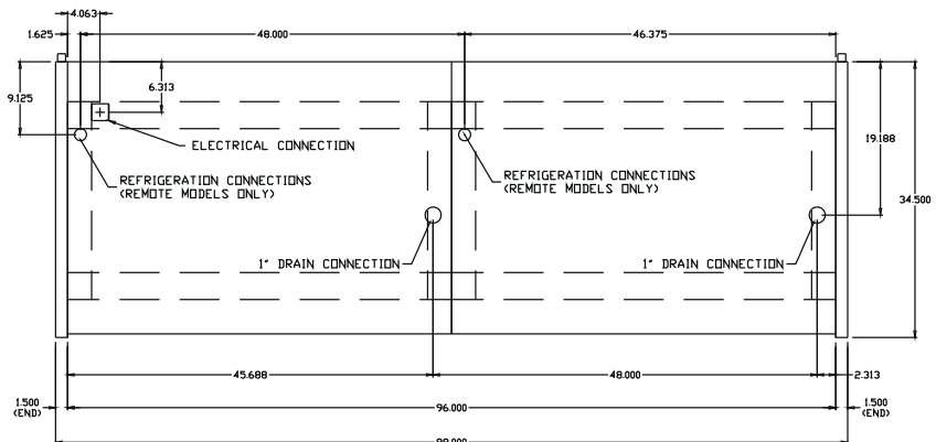
8' PLAN VIEW
