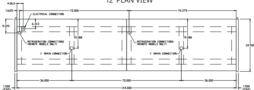
12' PLAN VIEW
